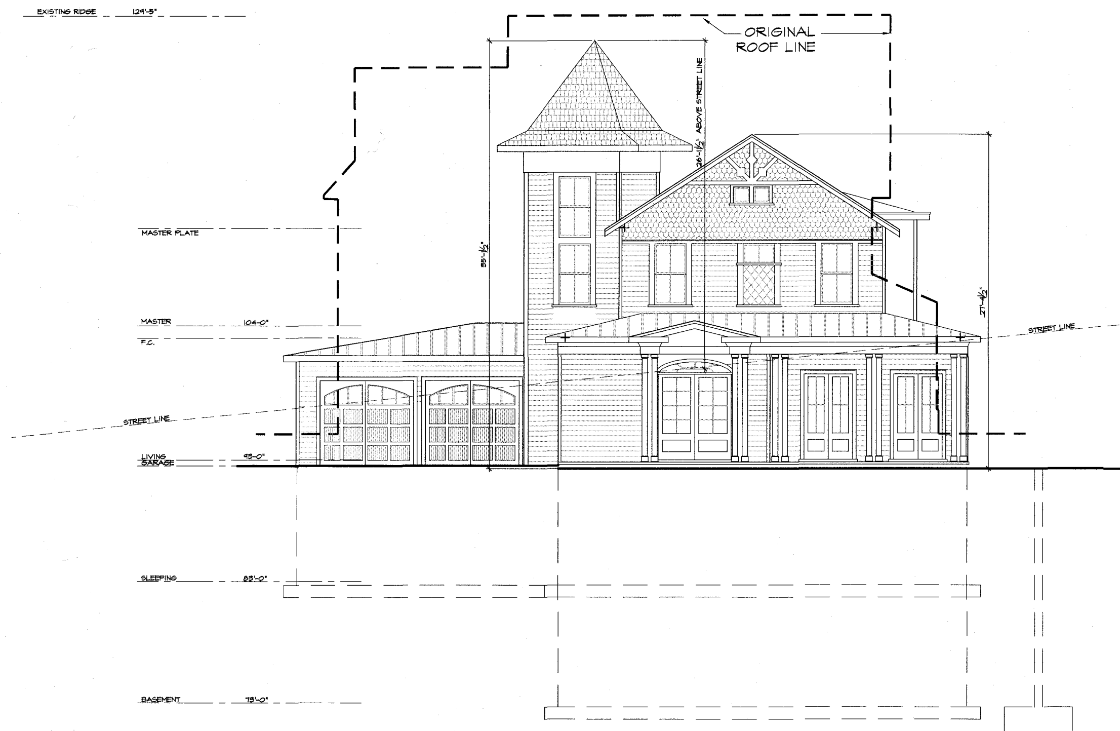
FRONT ELEV.
